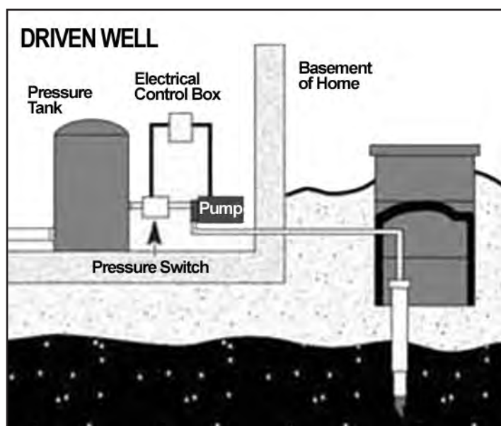
Figure 8.2. Cross Section of a Driven Well
