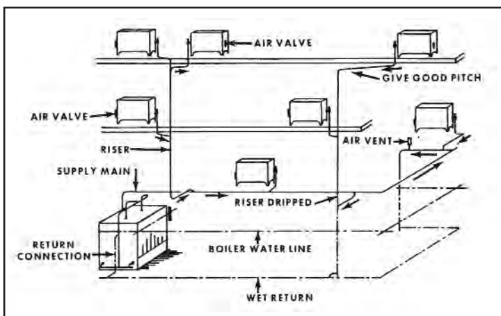
Figure 12.10. Typical Gravity One-pipe Heating System [4]
