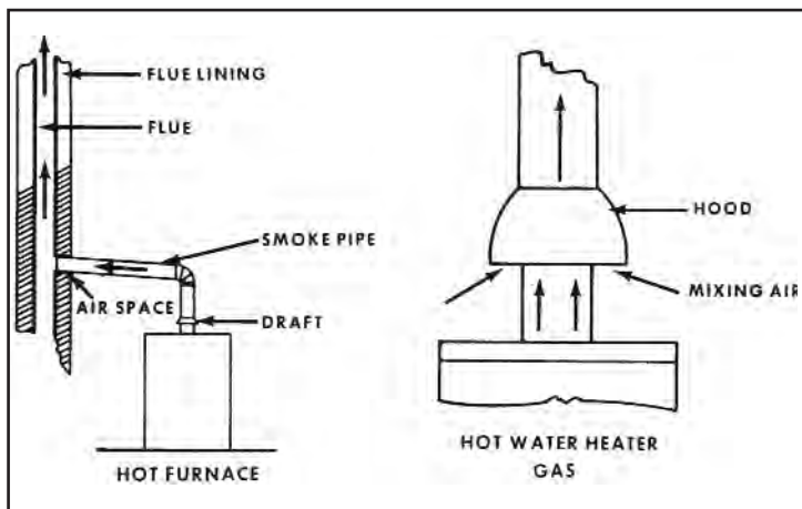
Figure 12.19. Location and Operation of Typical Backdraft Diverter [4]
