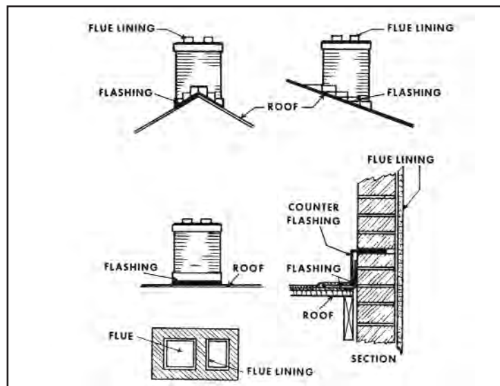
Figure 12.22. Chimney Plan [4]
