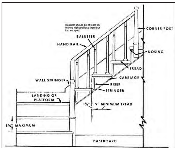
Figure 6.5. Interior Stairway [4]
