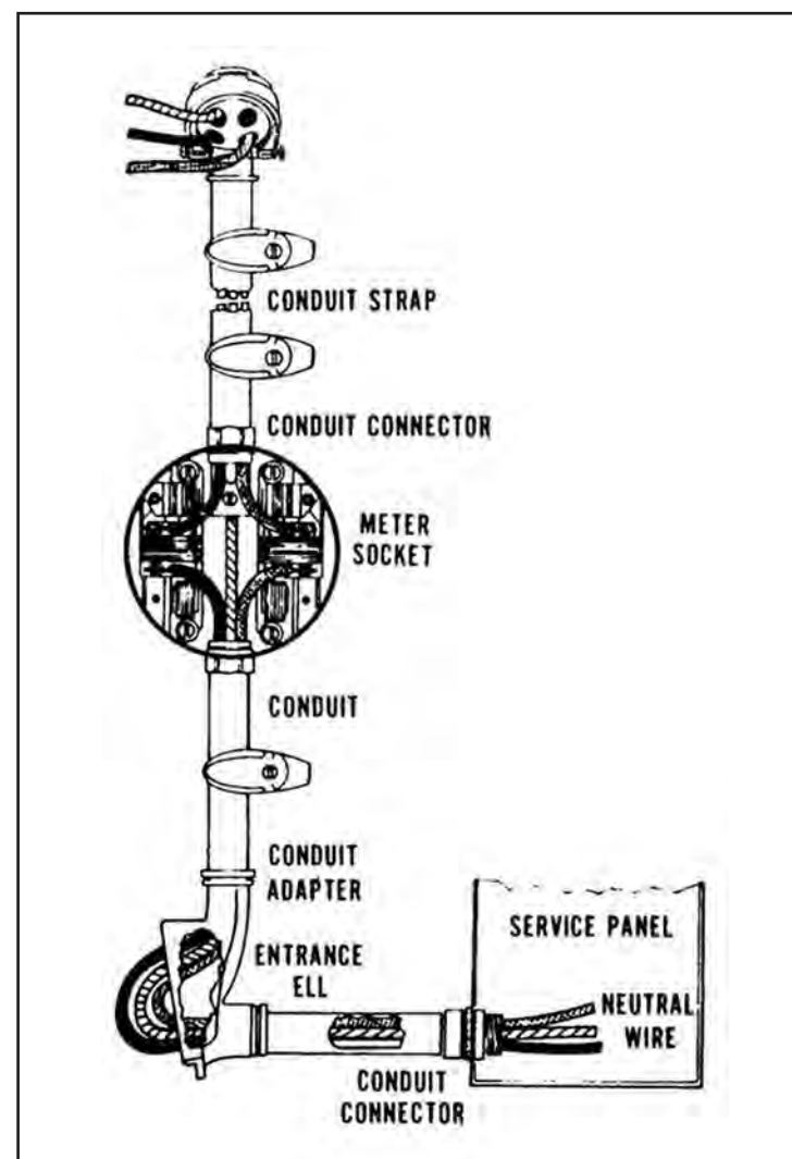
Figure 11.5. Thin-wall Conduit [2]
